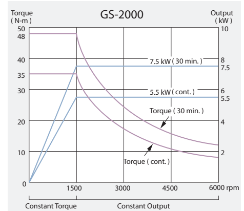
Sub-spindle Output
