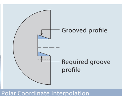
Grooving by Polar Coordinate Interpolation
